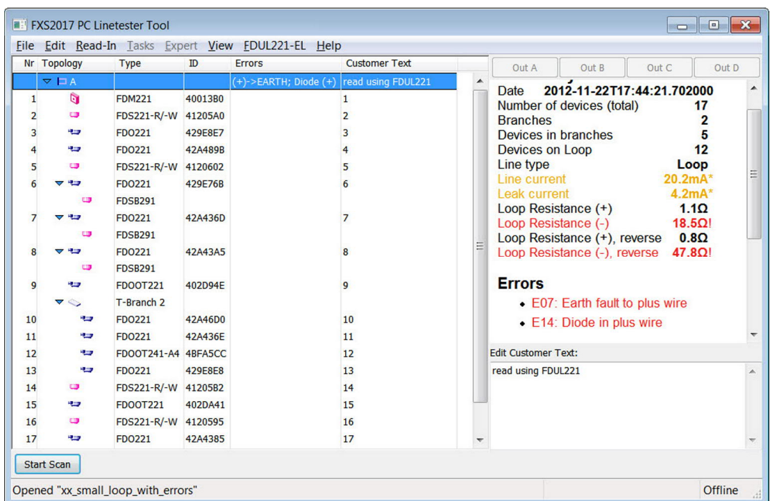
Line tester software FXS2017
